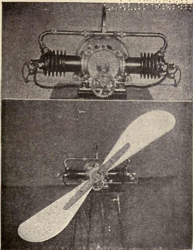
The interesting horizontal-opposed Jopson gasoline motor for model aéroplanes. The top photograph shows the half-speed shaft and the arrangement of the valve mechanism. This engine is air cooled, develops 1 h.p. at 1,500 r.p.m., and weighs 7\frac{1}{2} lbs., including gasoline tank and propeller. The bottom view shows the engine with propeller in situ . Courtesy Flight .
