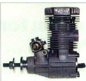
WEBRA 1.45 ABN PUMP
